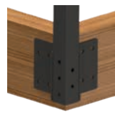
Fascia Post shown with brackets
